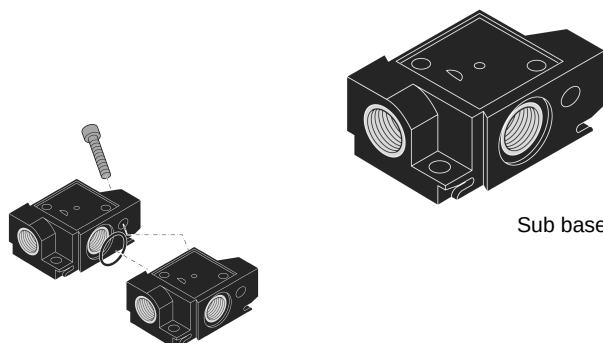
Modular Manifold System
