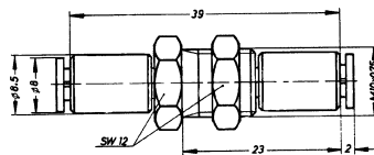
Bulkhead Coupling 52030
